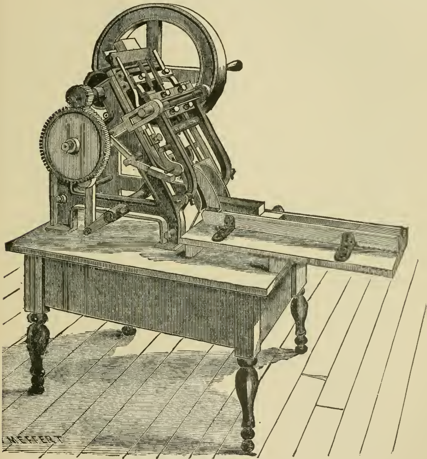
NUMBERING CARD PRESS.
